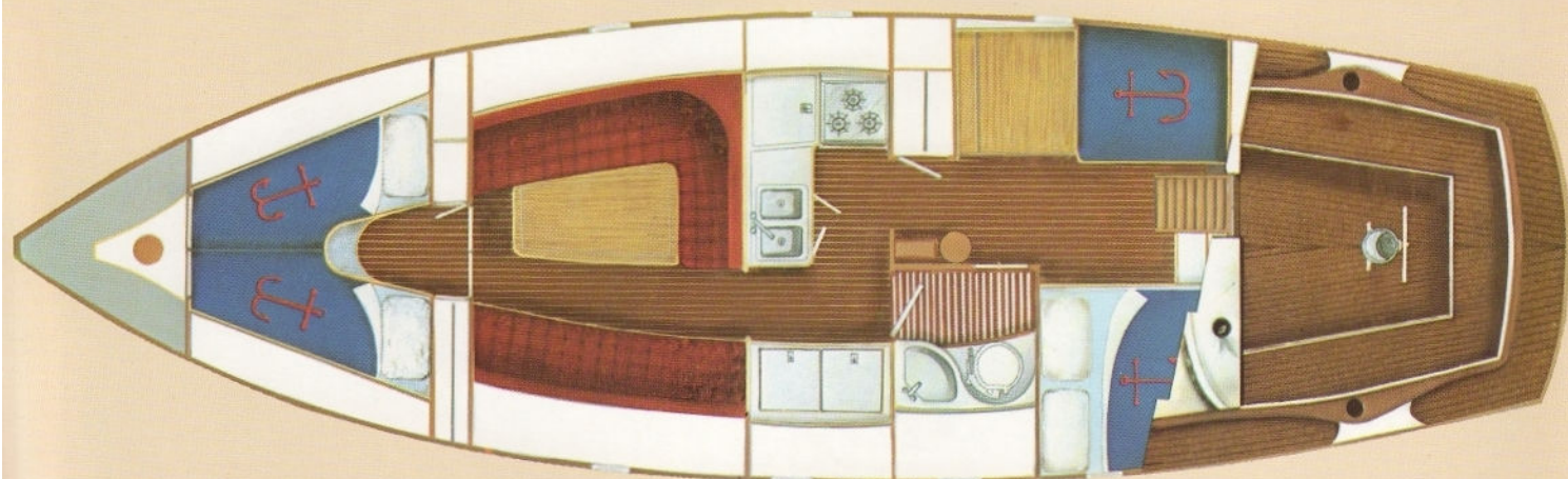
AFT COCKPIT
